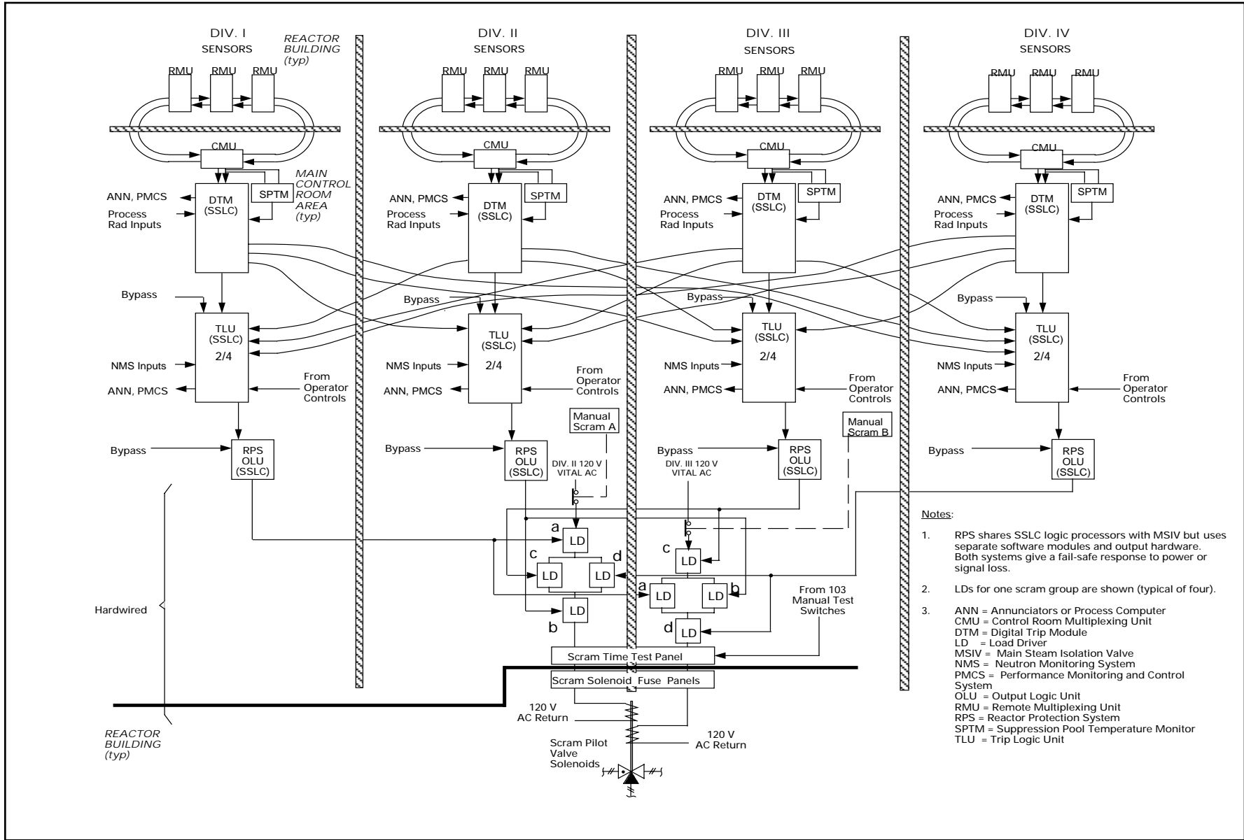
Figure 7.2-1 RPS Equipment Arrangement
