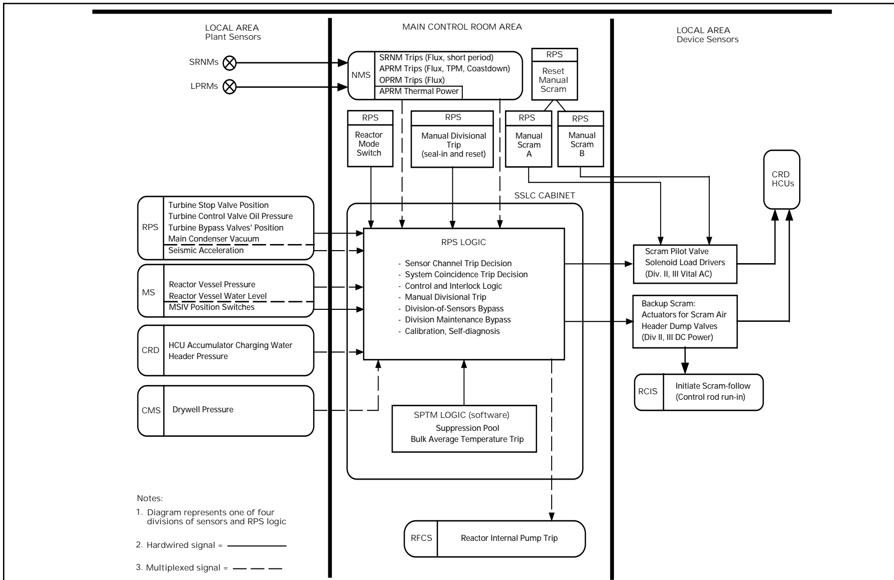
Figure 7.2-2 RPS Control Interface Diagram
