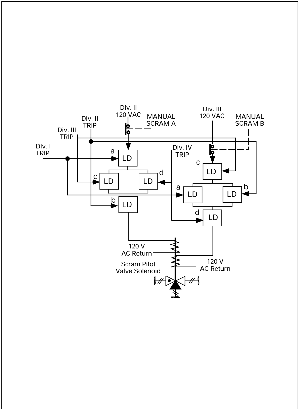
Figure 7.2-3 Scram Pilot Valve Solenoids Load Drivers Arrangement
